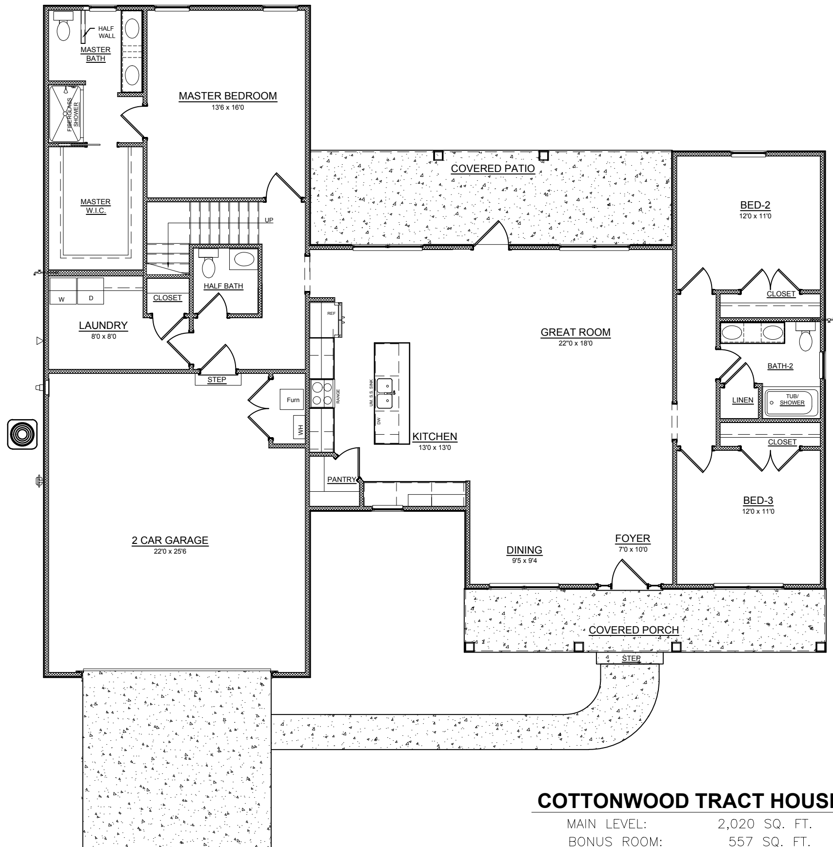
MAIN LEVEL PLAN
