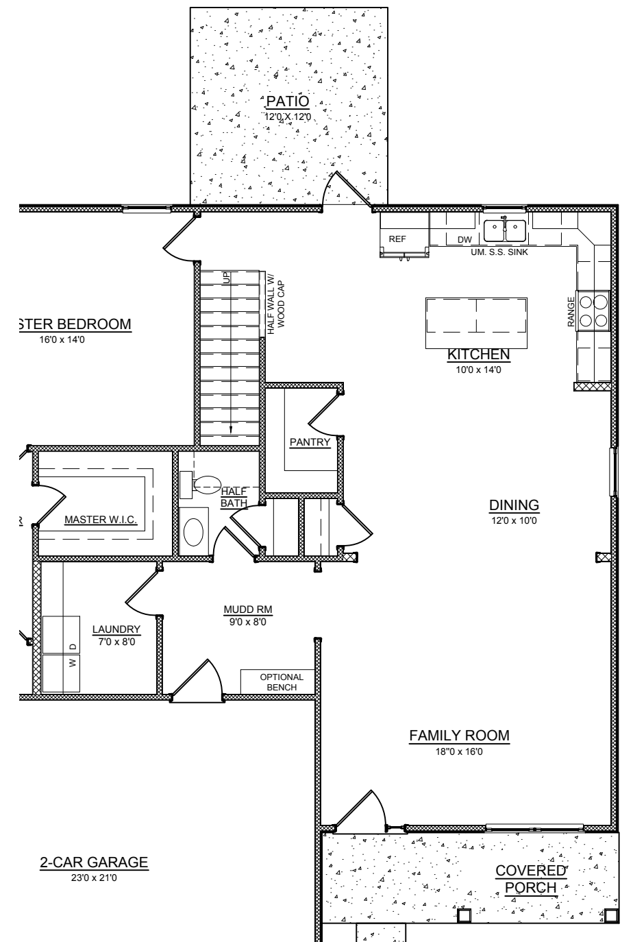
ALTERNATE MAIN LEVEL PLAN
