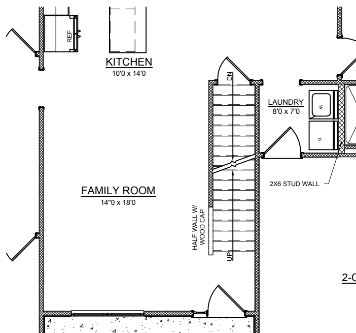
BASEMENT ACCESS PLAN
