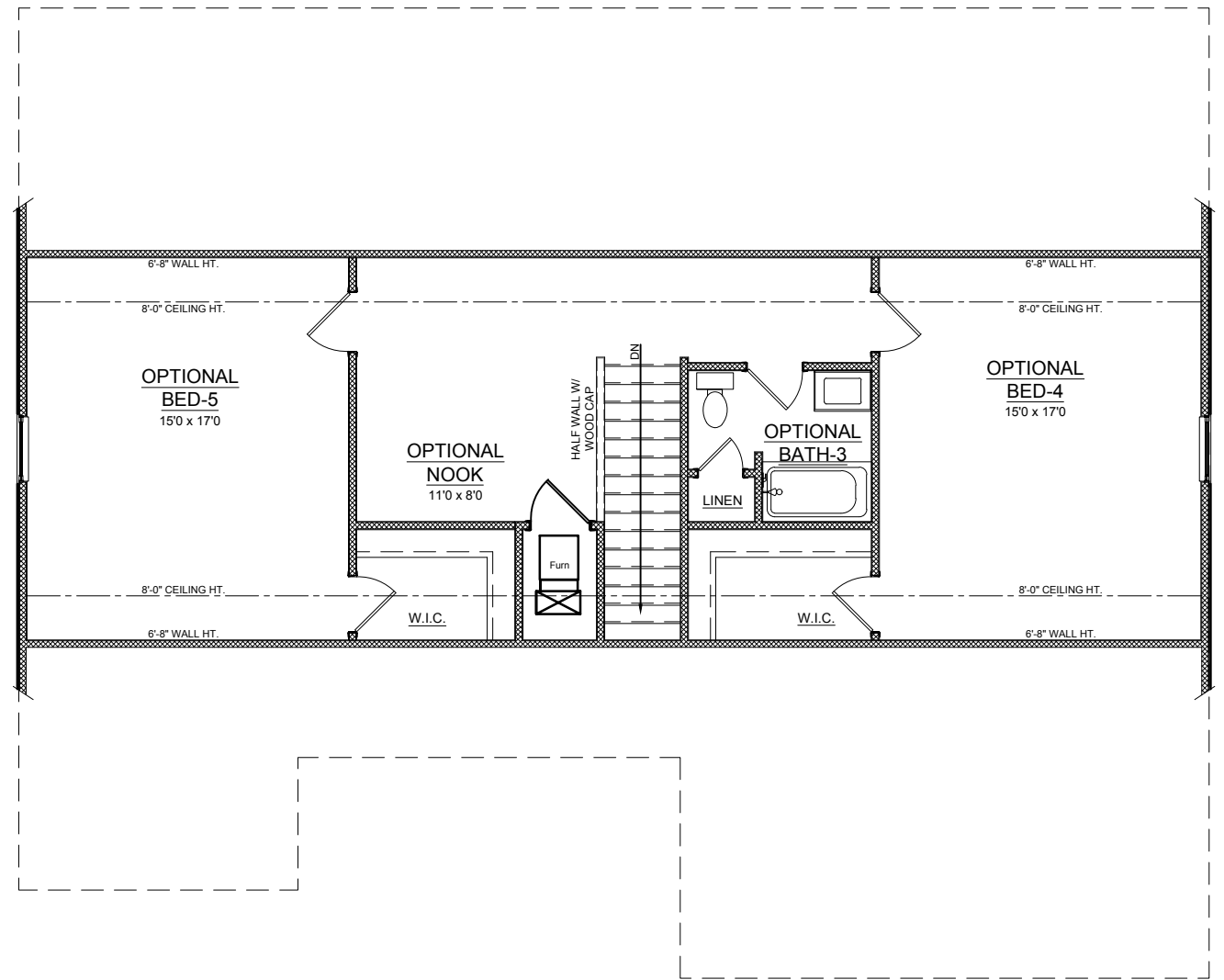
OPTION 2 ADD BEDROOM-5 UPPER LEVEL PLAN
