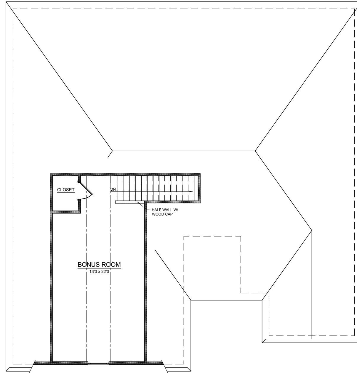
UPPER LEVEL PLAN
