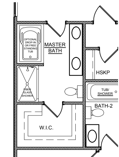
ADD MASTER TUB
