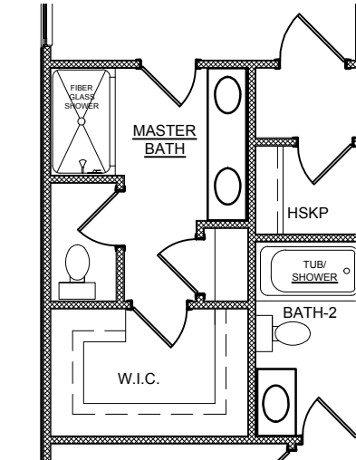
MASTER BATH OPTION
