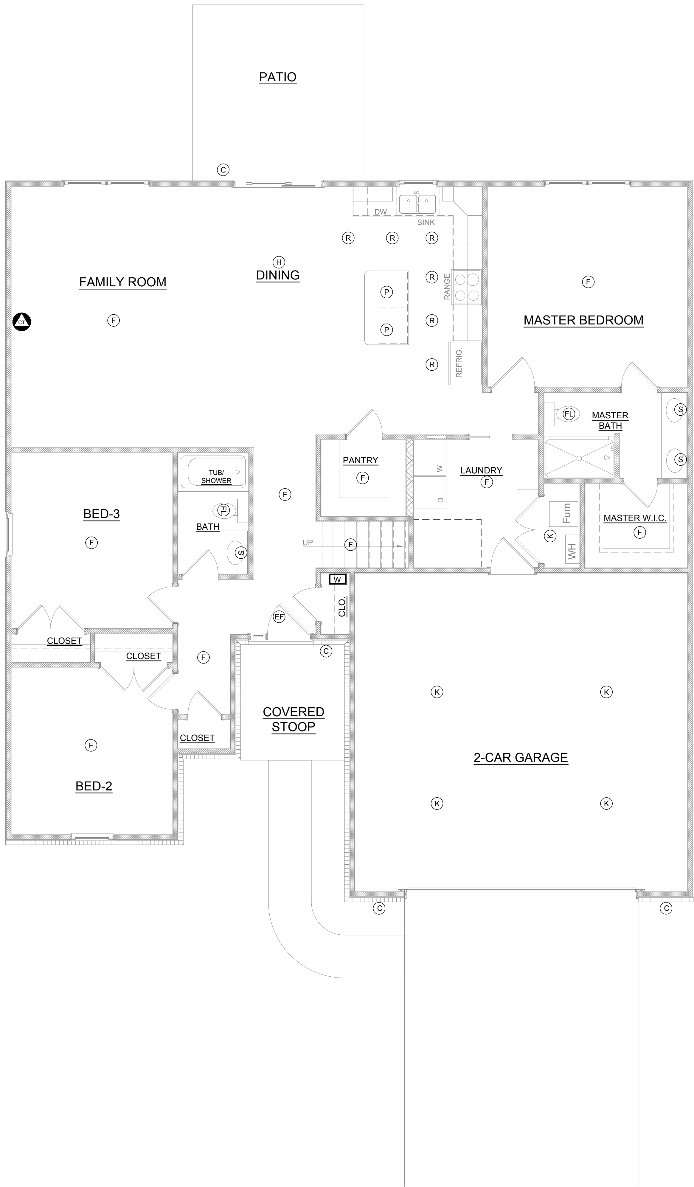
MAIN LEVEL ELECTRICAL PLAN SCALE: 1/4" = 1'-0"
