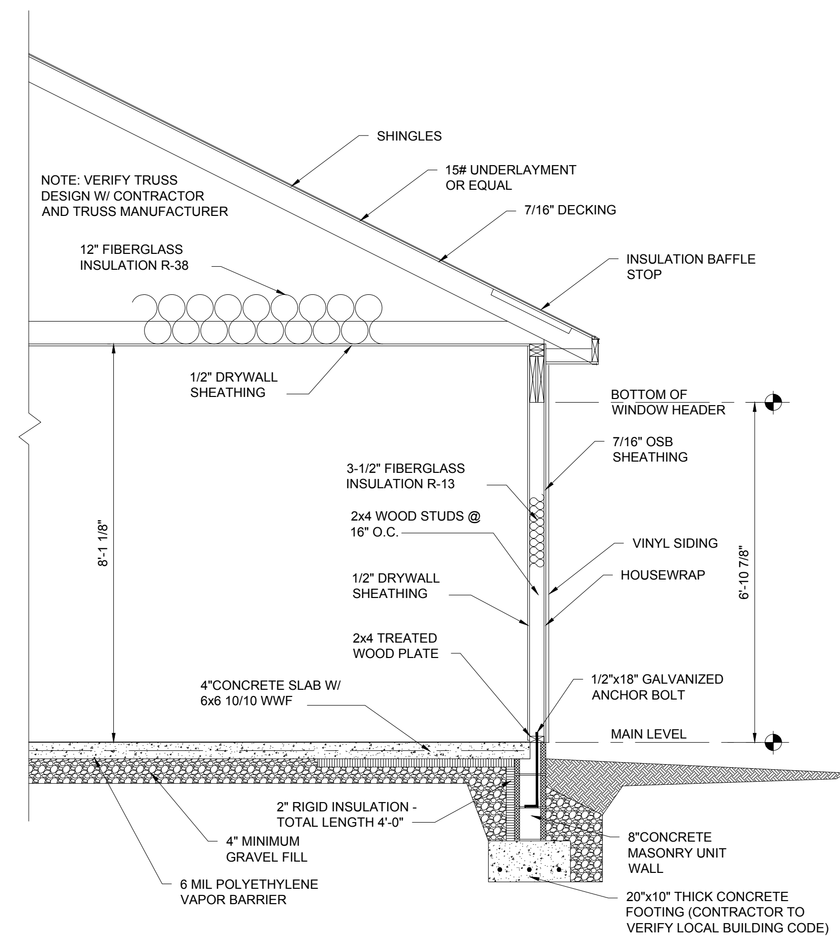
REAR & SIDE WALL SECTION SCALE: 3/4" = 1'-0"
