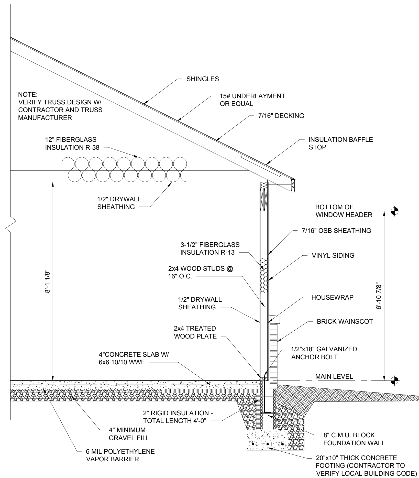
FRONT WALL SECTION SCALE: 3/4" = 1'-0"
