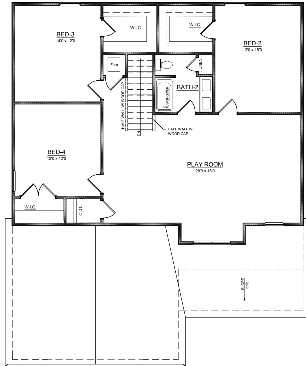
UPPER LEVEL PLAN MAPLE TRACT HOUSE:
