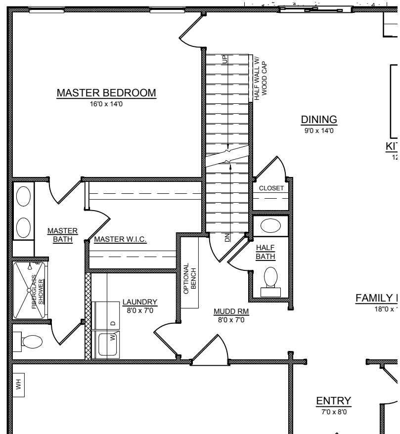
BASEMENT OPTION MAIN LEVEL PLAN
