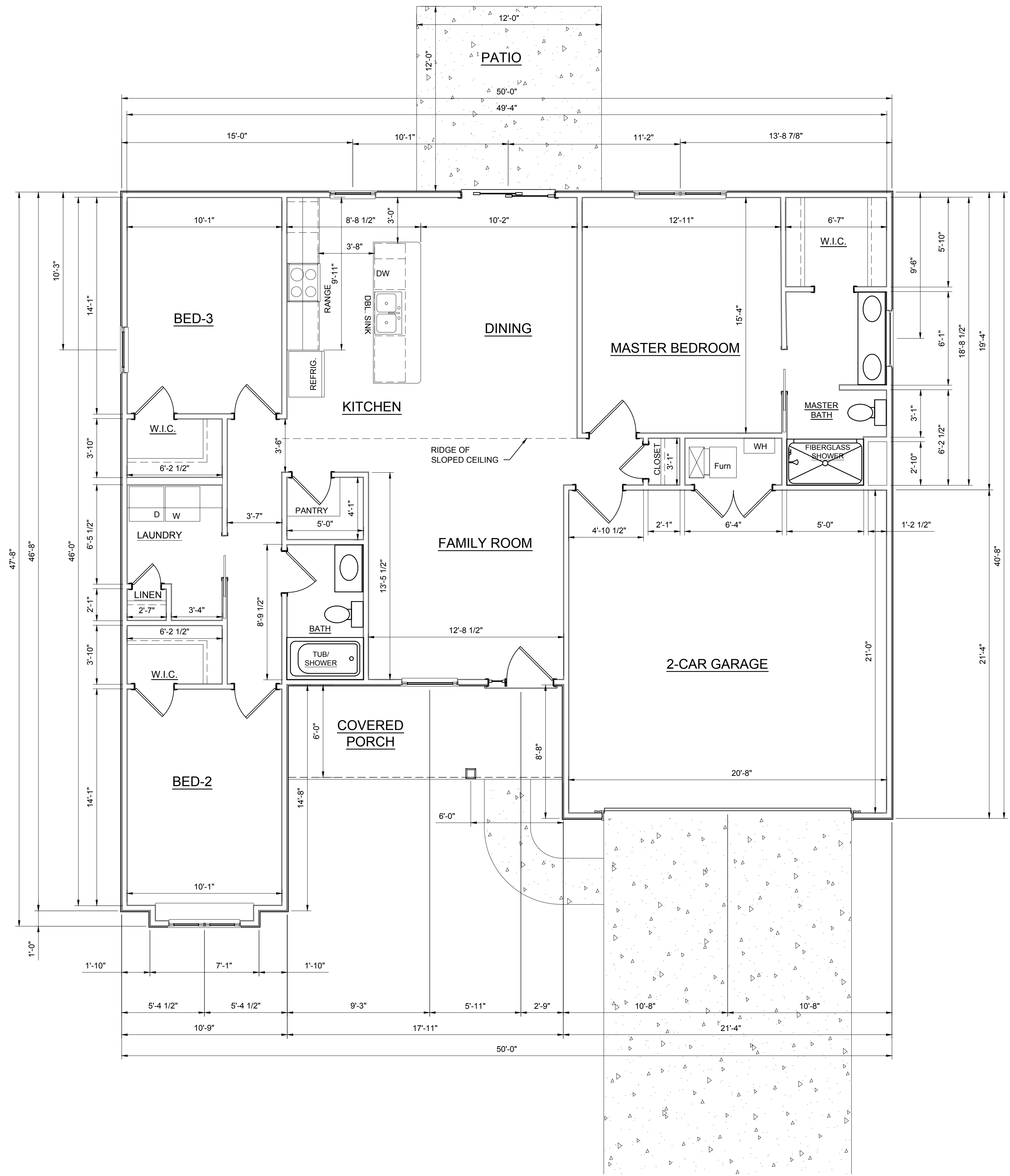
MAIN LEVEL PLAN SCALE: 1/4" = 1'-0"
