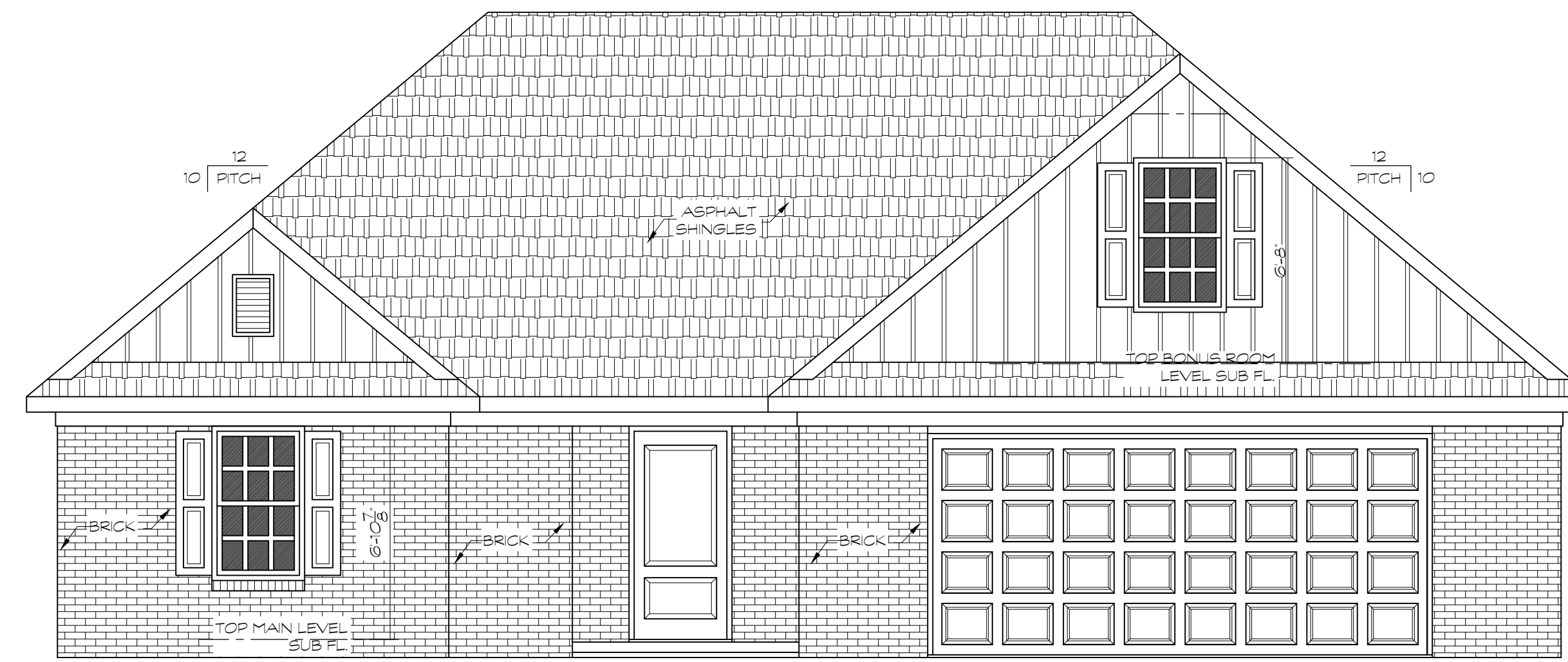
FRONT ELEVATION A
