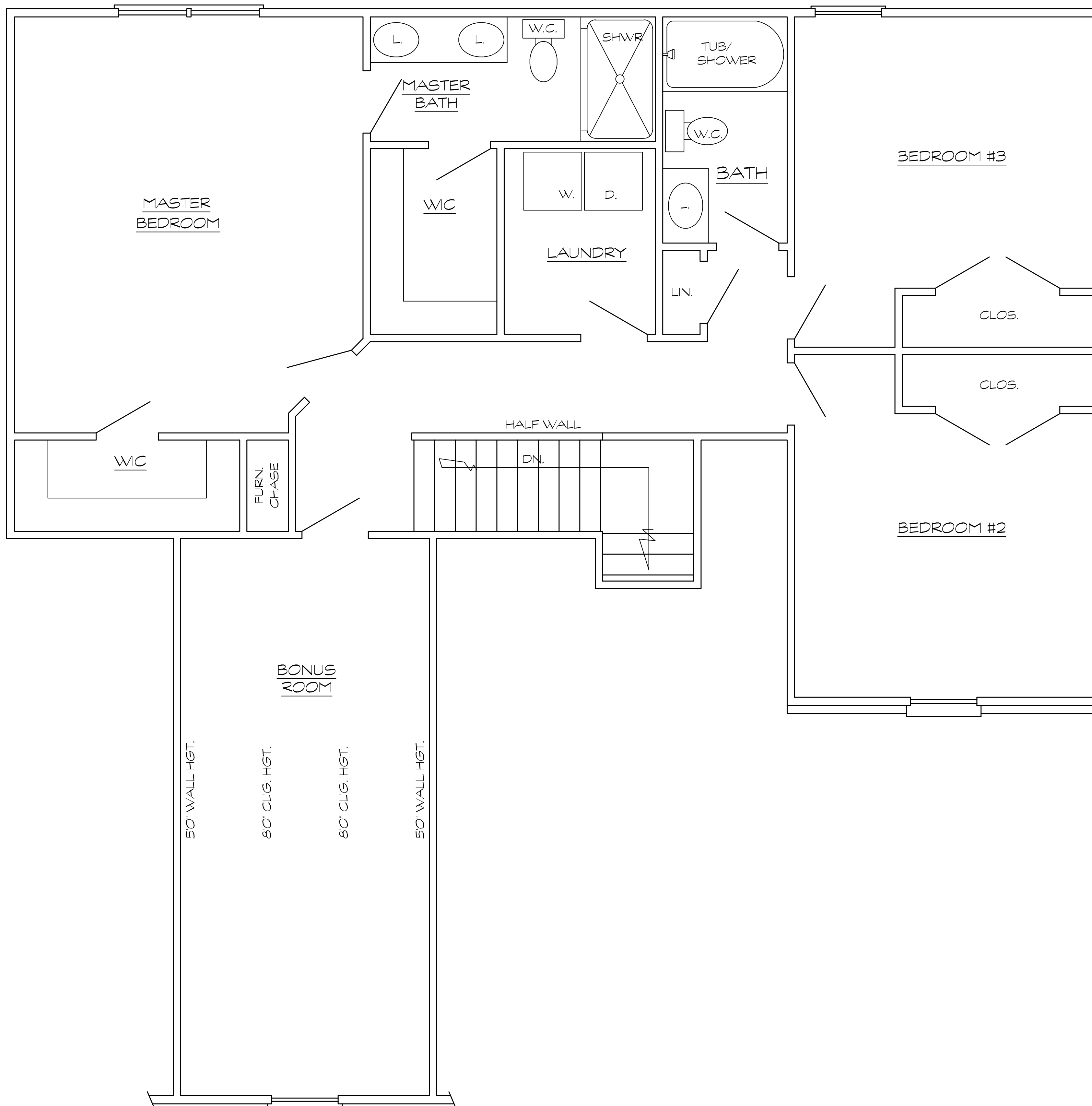
SECOND LEVEL FLOOR PLAN
