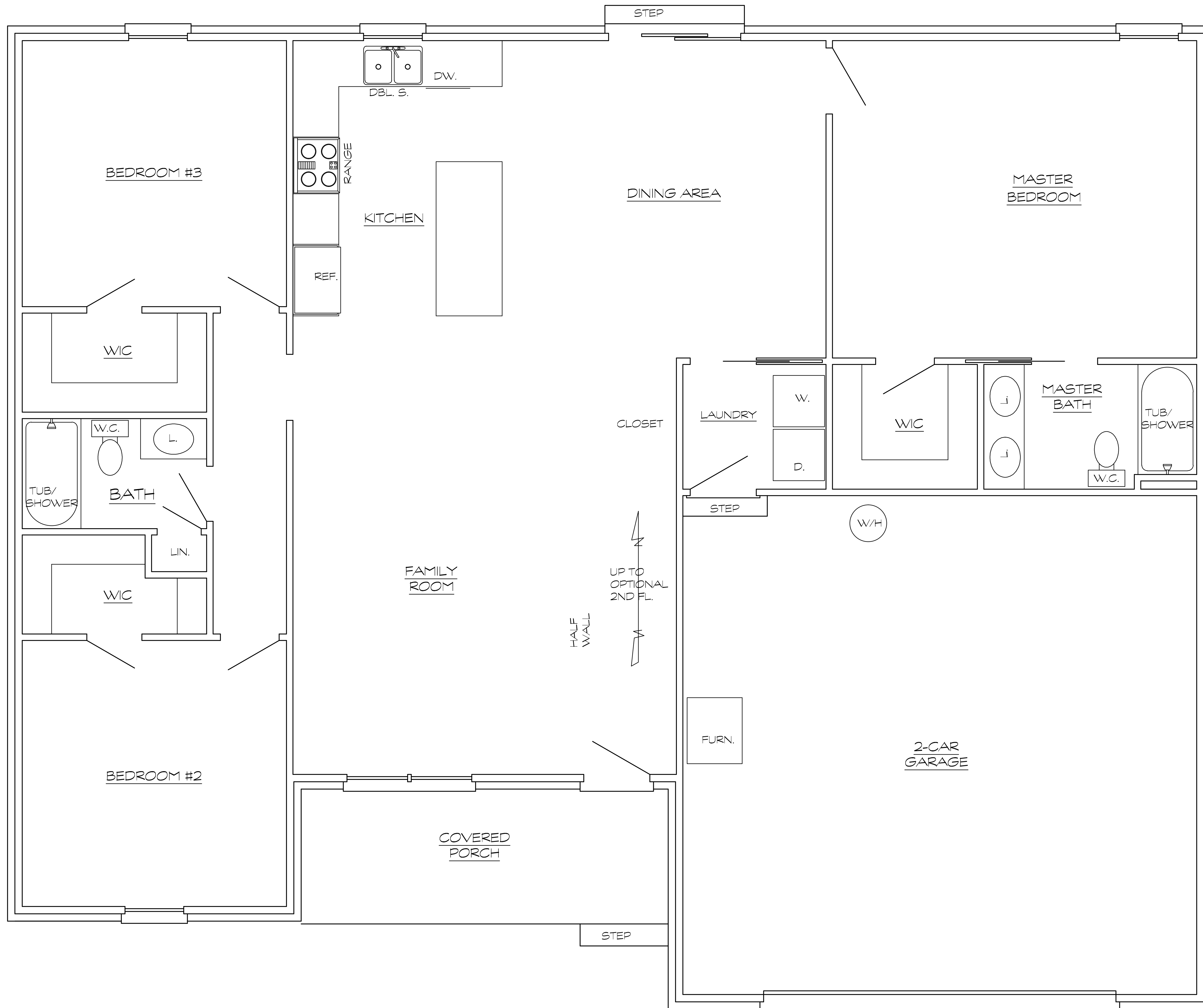
MAIN LEVEL FLOOR PLAN
