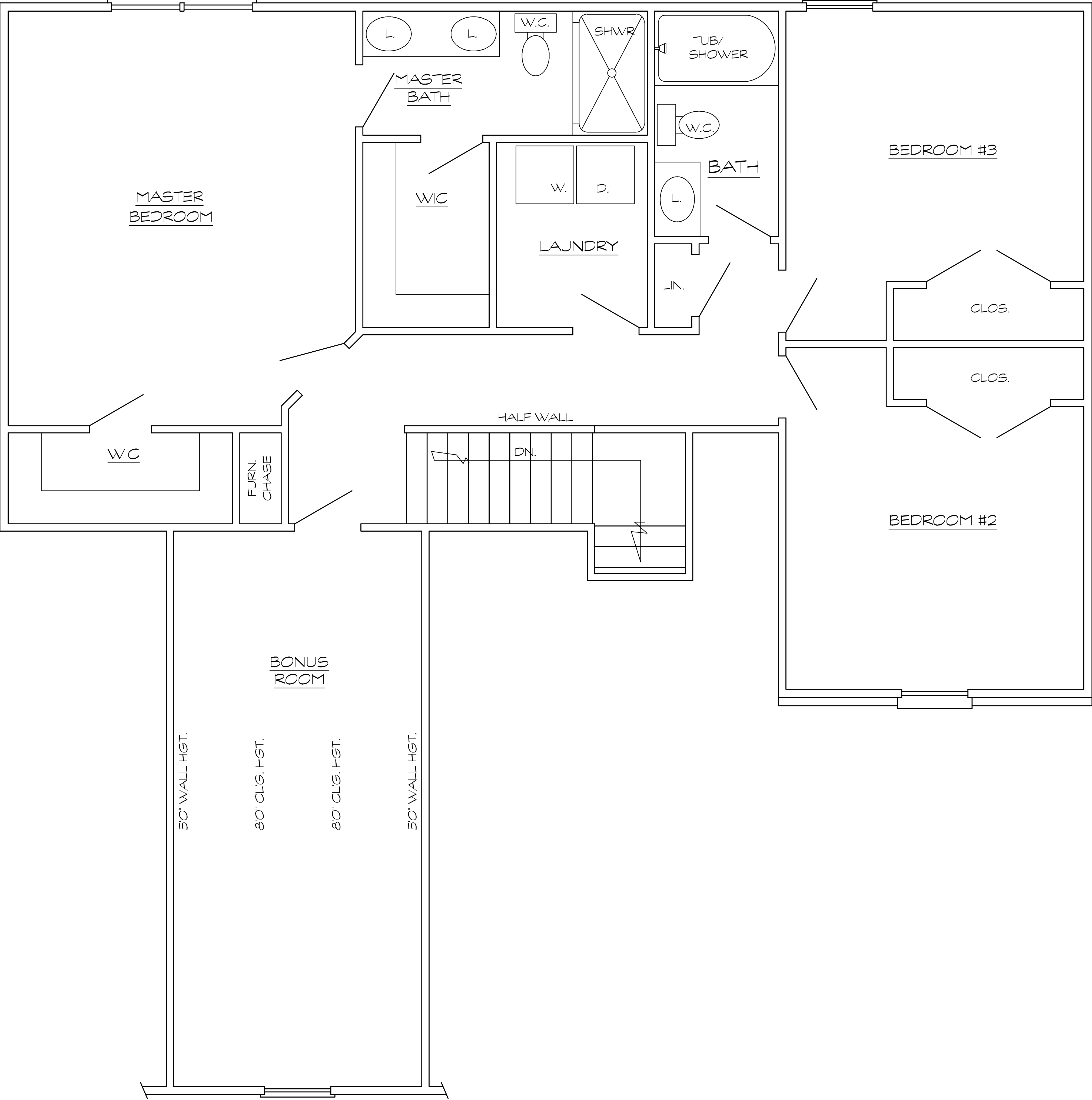
SECOND LEVEL FLOOR PLAN
